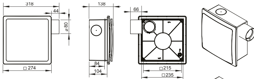
VNV-1 80 KV
