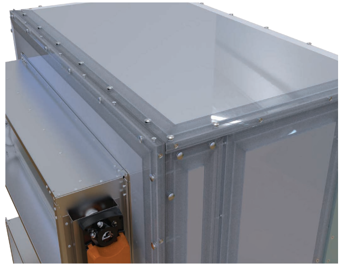
PVC profile system inside the unit casing
