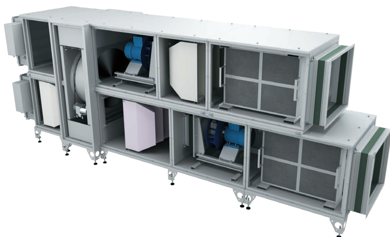
FRAMELESS DESIGN - AVF
