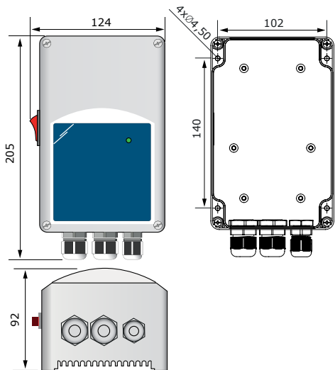
Fig. 1. Dimensions [mm]
